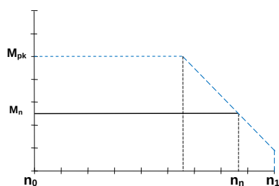
TORQUE DIAGRAM
